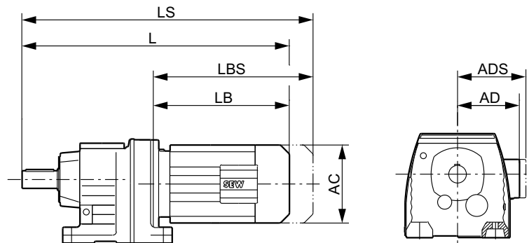
Figure 29: Dimension designations for the motors
