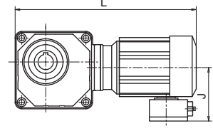
Fig. 4 0.2~0.4kW Without brake
