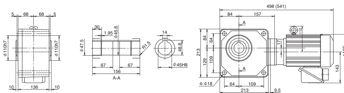
Fig. 4 Designate model and voltage and frequency when ordering. Brackets contain dimension, model, or mass of type with brakes. RNYM1-1530-80-240 Mass 25kg (RNYM1-1530-B-80-240) (Mass 28kg)
