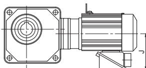
Fig. 4 0.4~1.5kW Without brake
