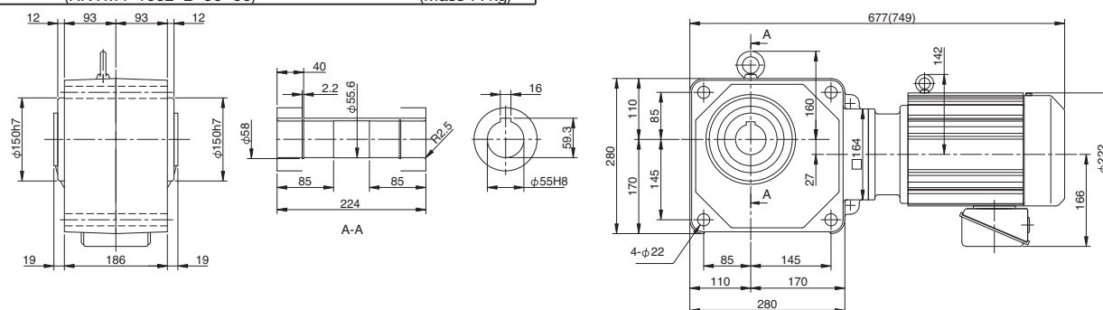
Fig. 4 RNYM4-1632-30-60 (RNYM4-1632-B-30~60) Mass 66kg (Mass 77kg)
