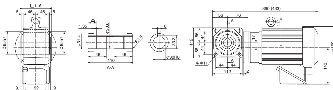
Fig. 4 RNYM1-1320-5~10 Mass 15kg (RNYM1-1320-B-5~10) (Mass 17kg)
