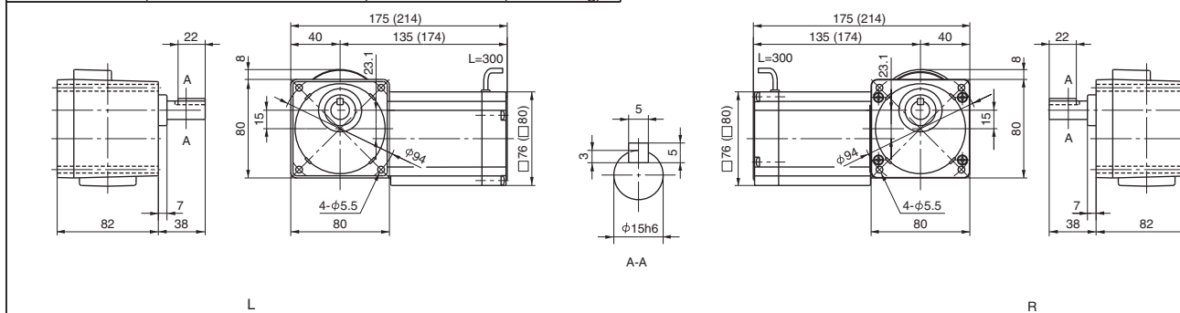
Fig. 4 RNFM0025-03 B-80-240 Mass 2.9kg (RNFM0025-03 B-B-80-240) (Mass 3.5kg)
