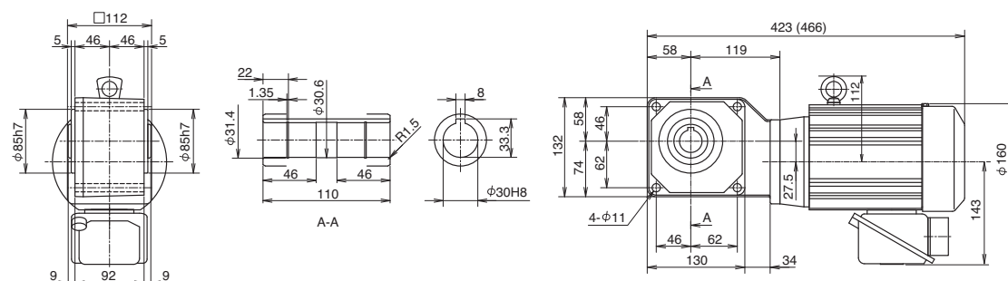
Fig. 4 RNYM1-1320-5~10 Mass 15kg (RNYM1-1320-B-5~10) (Mass 17kg)
