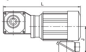
Fig. 2 0.2~0.4kW Without brake
