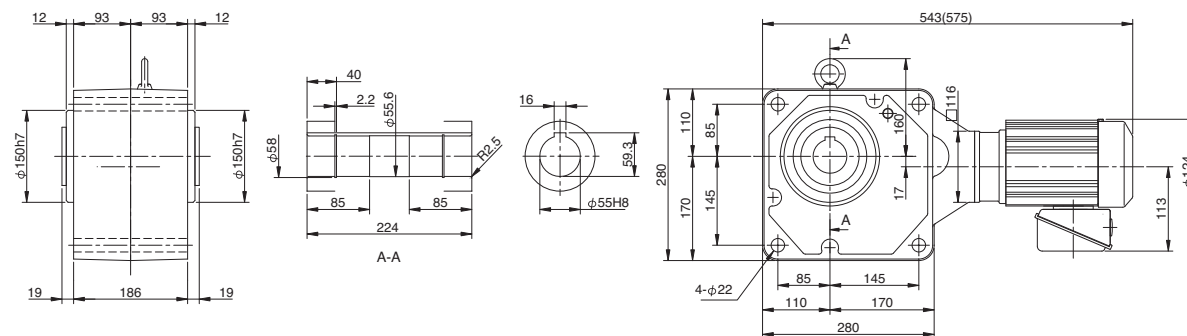
Fig. 2 RNYM05-1640-300~1440 (RNYM05-1640-B-300~1440) Mass 63kg (Mass 64kg)
