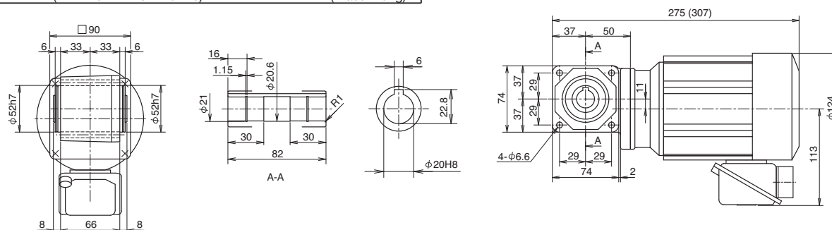
Fig. 3 Designate model and voltage and frequency when ordering. Brackets contain dimension, model, or mass of type with brakes. RNYM02-1110-5-10 (RNYM02-1110-B-5-10) Mass 6.0kg (Mass 7.5kg)
