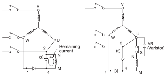
Fig. 15 standard circuit
