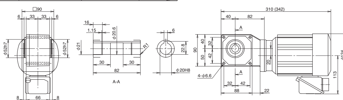
Fig. 4 RNYM02-1120-5-10 (RNYM02-1120-B-5-10) Mass 7.0kg (Mass 8.5kg)
