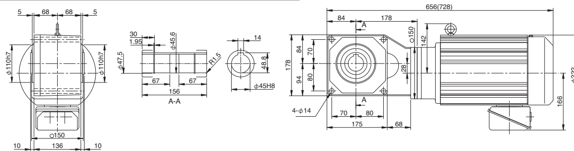
Fig. 1 Designate model and voltage and frequency when ordering. Brackets contain dimension, model, or mass of type with brakes. RNYM8-1522-5~15 (RNYM8-1522-B-5~15) Mass 57kg (Mass 68kg)
