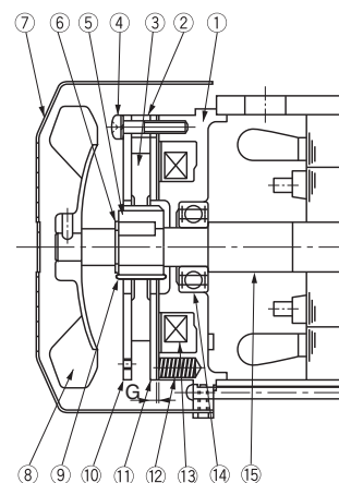
Fig. 22 FB-01A1,02A1,05A1 (0.1kW~0.4kW×4 Poles) (FB-01A1 Without Fan)
