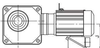
Fig. 6 Without brake
