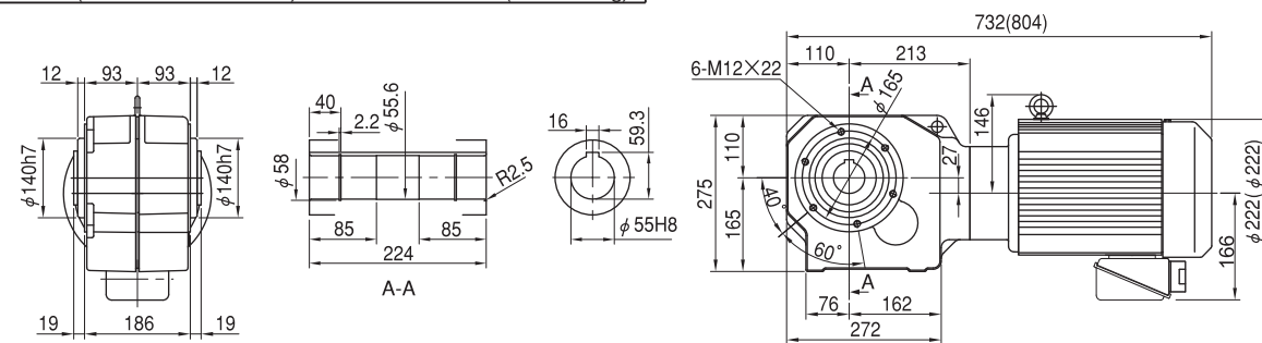
Fig. 3 RNYM8-1634-5~25 (RNYM8-1634-B-5~25) Mass 95kg (Mass 105kg)
