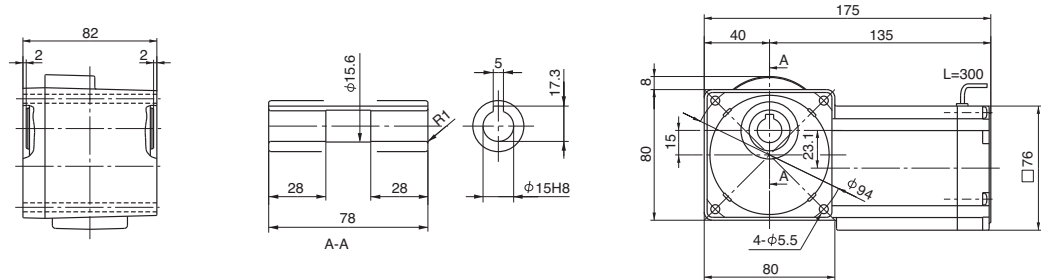
Fig. 2 Designate model and voltage and frequency when ordering. → RNYM0025-03-CC-5~240 Mass 2.7kg
