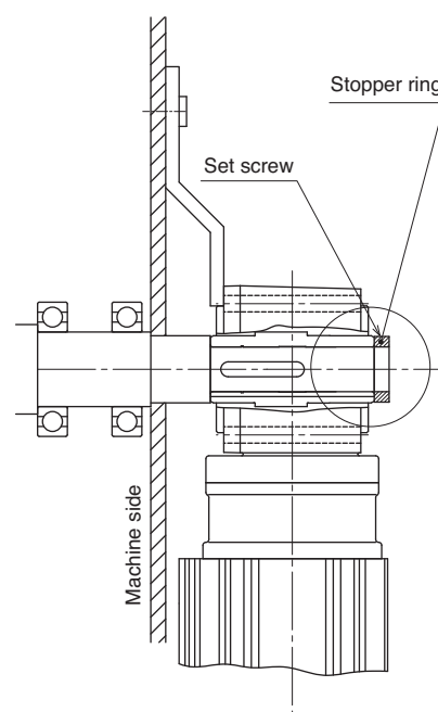
Fig. 7 secured by a set screw and a stopper ring
