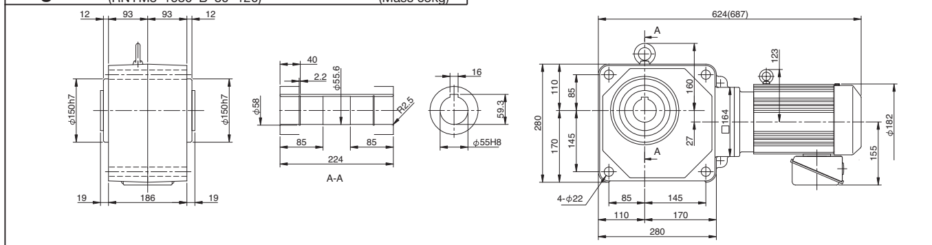
Fig. 4 Designate model and voltage and frequency when ordering. Brackets contain dimension, model, or mass of type with brakes. RNYM3-1630-80~120 (RNYM3-1630-B-80~120) Mass 57kg (Mass 63kg)
