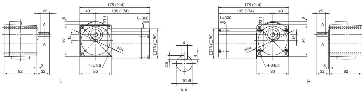
Fig. 1 Designate model and voltage and frequency when ordering. Brackets contain dimension, model, or mass of type with brakes. RNFM0015-01 CA-5~100 Mass 2.7kg (RNFM0015-01 CA-B-5~100) (Mass 3.3kg)
