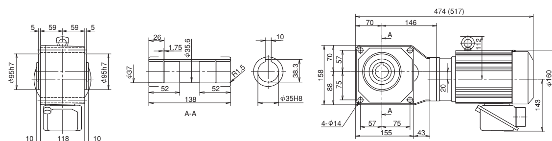
Fig. 5 RNYM1-1420-5~10 Mass 18kg (RNYM1-1420-B-5~10) (Mass 20kg)
