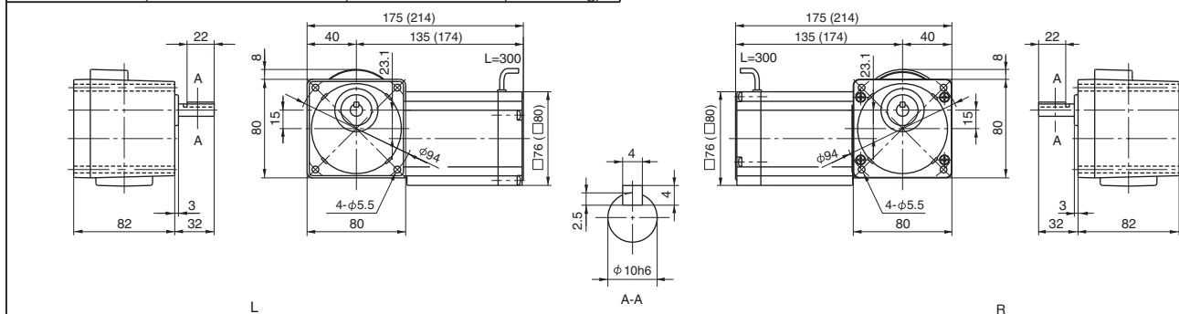
Fig. 3 Designate model and voltage and frequency when ordering. Brackets contain dimension, model, or mass of type with brakes. RNFM0025-01 B-5-60 Mass 2.8kg (RNFM0025-01 B-B-5-60) (Mass 3.4kg)
