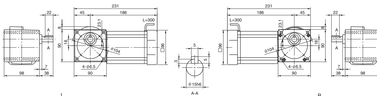
Fig. 4 Designate model and voltage and frequency when ordering. RNFM006-15 \frac{1}{2} -CC-5-60 MassA 4.5kg
