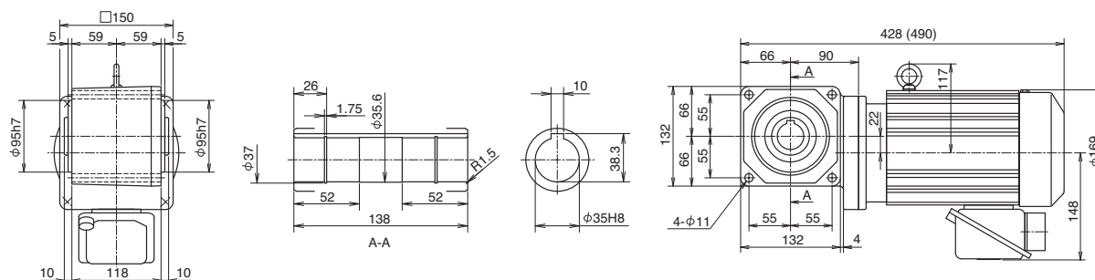
Fig. 4 Designate model and voltage and frequency when ordering. Brackets contain dimension, model, or mass of type with brakes. RNYM2-1410-5~10 (RNYM2-1410-B-5~10) Mass 22kg (Mass 26kg)
