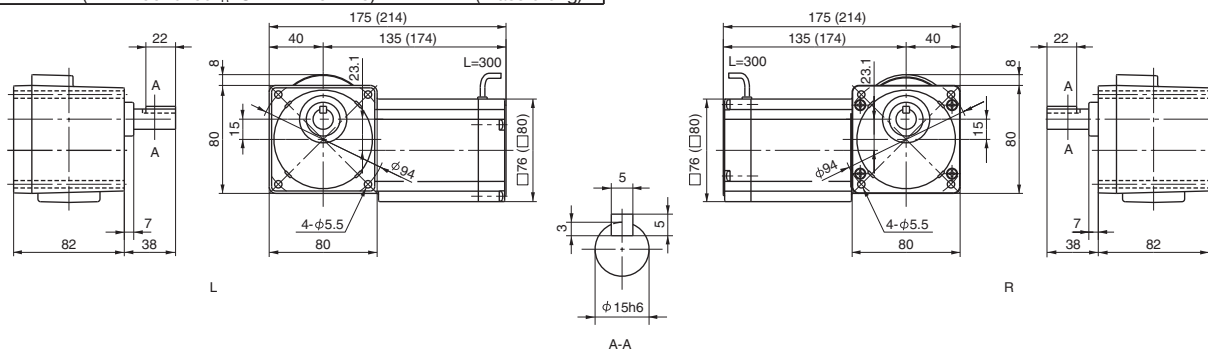
Fig. 2 RNFM0015-03 CA-120~240 Mass 2.7kg (RNFM0015-03 CA-B-120~240) (Mass 3.3kg) • Use hex socket head cap screws (M5) for installation.
