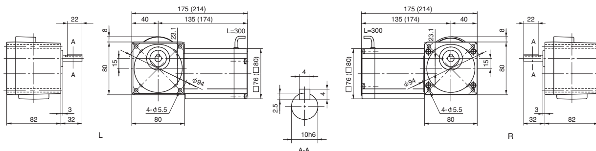
Fig. 3 Designate model and voltage and frequency when ordering. Brackets contain dimension, model, or mass of type with brakes. RNFM0025-01 CA-5-60 Mass 2.8kg (RNFM0025-01 CA-B-5-60) (Mass 3.4kg)
