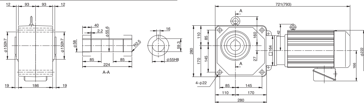
Fig. 3 RNYM8-1634-5~25 (RNYM8-1634-B-5~25) Mass 95kg (Mass 105kg)
