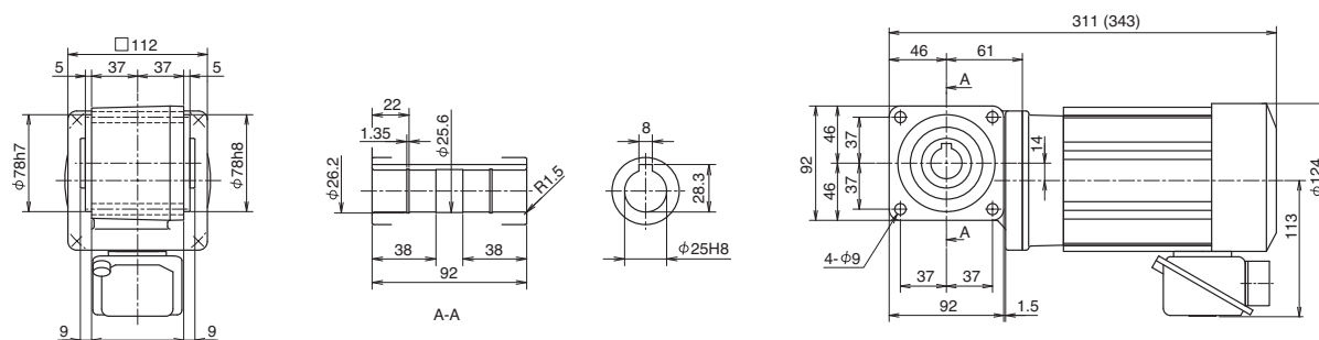
Fig. 3 Designate model and voltage and frequency when ordering. Brackets contain dimension, model, or mass of type with brakes. RNYM03-1210-5-10 (RNYM03-1210-B-5~10) Mass 9.0kg (Mass 10kg)
