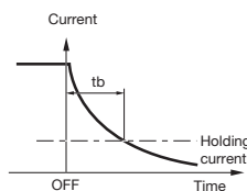
Fig. 17 current curve of standard braking circuit
