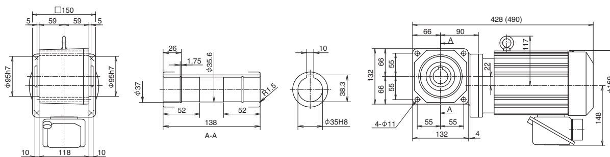
Fig. 4 Designate model and voltage and frequency when ordering. Brackets contain dimension, model, or mass of type with brakes. RNYM1H-1410-5~10 (RNYM1H-1410-B-5~10) Mass 20kg (Mass 24kg)
