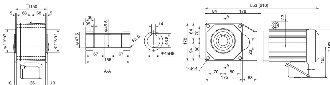
Fig. 1 Designate model and voltage and frequency when ordering. Brackets contain dimension, model, or mass of type with brakes. RNYM3-1520-5-30 (RNYM3-1520-B-5-30) Mass 34kg (Mass 39kg)
