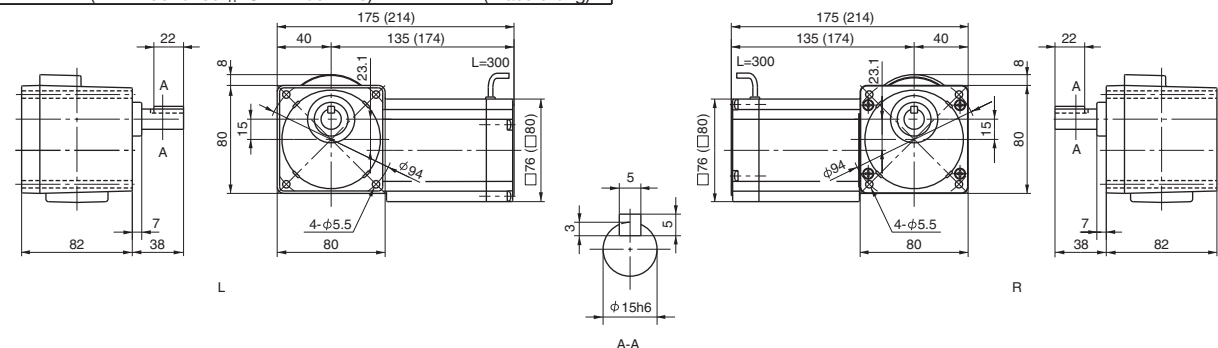
Fig. 4 RNFM0025-03 CA-80-240 Mass 2.9kg (RNFM0025-03 CA-B-80-240) (Mass 3.5kg)
