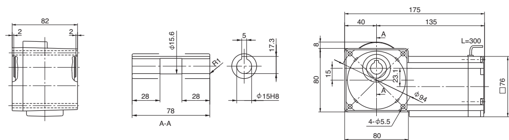
Fig. 1 Designate model and voltage and frequency when ordering. → RNYM0015-03-CC-5-240 Mass 2.6kg
