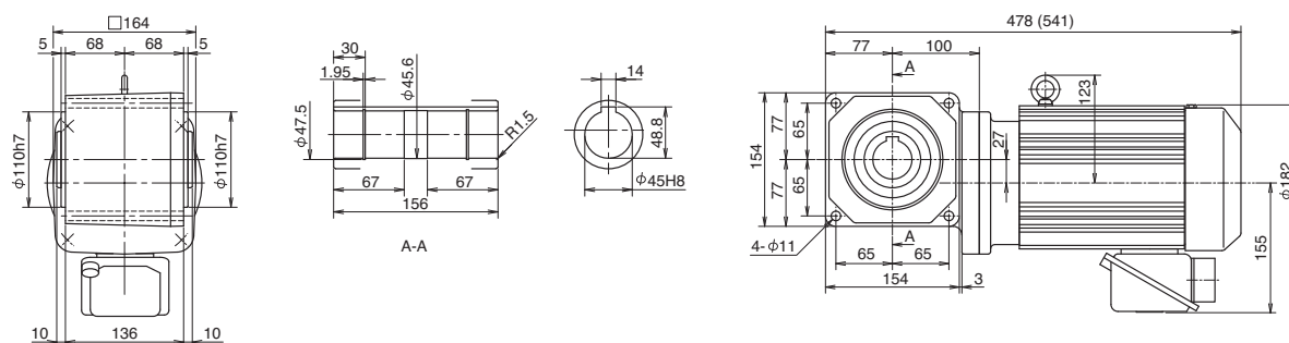
Fig. 4 Designate model and voltage and frequency when ordering. Brackets contain dimension, model, or mass of type with brakes. RNYM3-1510-5~10 (RNYM3-1510-B-5~10) Mass 29kg (Mass 35kg)
