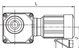
Fig. 2 0.1~0.2kW Without brake
