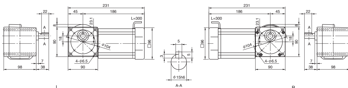
Fig. 1 Designate model and voltage and frequency when ordering. RNFM009-15 \frac{1}{2} -CC-5-60 Mass 5.0kg
