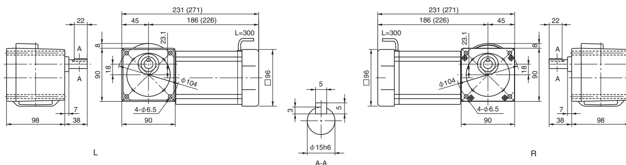
Fig. 1 Designate model and voltage and frequency when ordering. Brackets contain dimension, model, or mass of type with brakes. RNFM009-15 \frac{1}{2} -CA-5-60 Mass 5.0kg (RNFM009-15 \frac{1}{2} -CA-B-5-60) (Mass 5.4kg)
