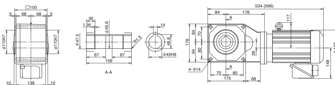
Fig. 6 RNYM1H-1520-40~60 (RNYM1H-1520-B-40~60) Mass 29kg (Mass 33kg)
