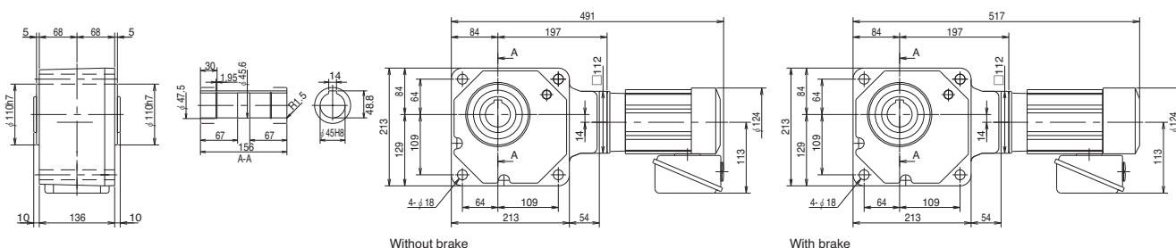
Fig. 1 Designate model and voltage and frequency when ordering. Brackets contain dimension, model, or mass of type with brakes. RNYM05-1540-300~1440 (RNYM05-1540-B-300~1440) Mass 26kg (Mass 27.5kg)
