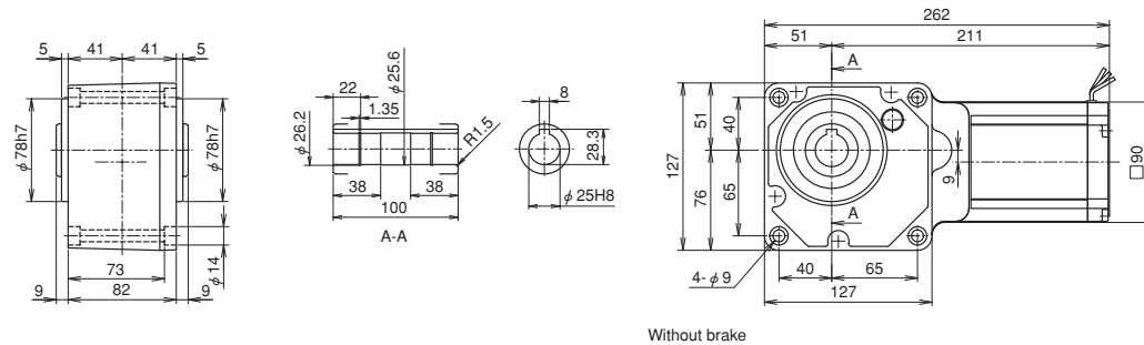
Fig. 3 Designate model, voltage, and frequency when ordering. RNYM004-1240-CC-300~1440 Mass 6.9kg
