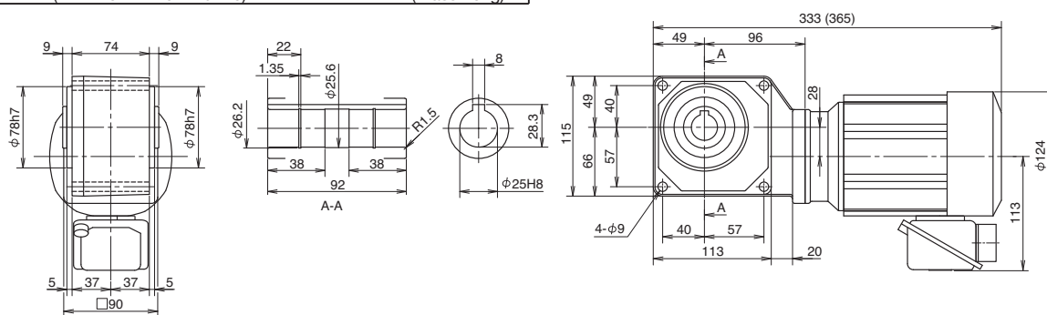
Fig. 5 RNYM02-1220-5-10 (RNYM02-1220-B-5-10) Mass 8.5kg (Mass 10kg)
