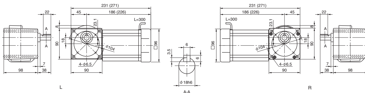
Fig. 2 RNFM009-17 \frac{1}{2} -CA-80-240 Mass 5.0kg (RNFM009-17 \frac{1}{2} -CA-B-80-240) (Mass 5.4kg)
