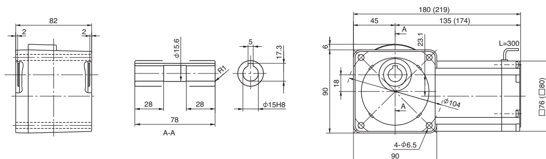
Fig. 1 Designate model and voltage and frequency when ordering. Brackets contain dimension, model, or mass of type with brakes. RNYM004-07-5~120 (RNYM004-07-B-5~120) Mass 2.9kg (Mass 3.5kg)
