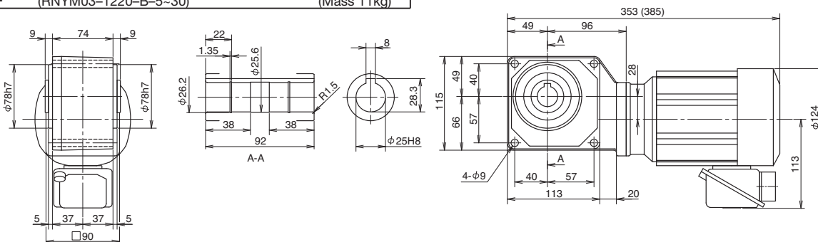
Fig. 4 RNYM03-1220-5-30 (RNYM03-1220-B-5~30) Mass 9.5kg (Mass 11kg)
